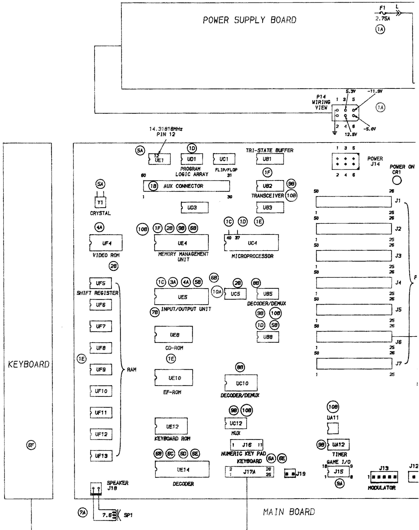
INTERCONNECTING DIAGRAM
